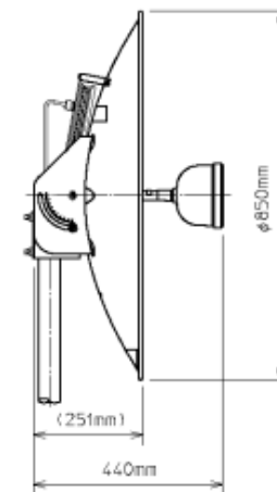
概略寸法 (Dimensions)
